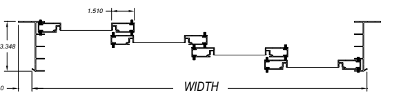
INSIDE MOUNT FRAME - 4-TRACK
