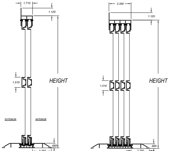
INSIDE MOUNT FRAME - 2-TRACK
